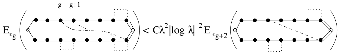
Figure 15: Case 3. Removal of two opposite lumped gates
