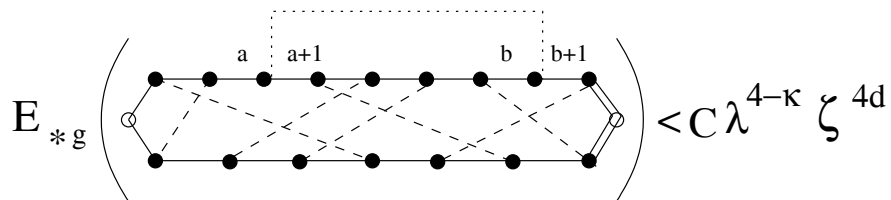
Figure 7: Estimate of a two-sided recollision graph
