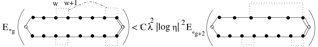
Figure 13: Case 2. Removal of two adjacent lumped gates
