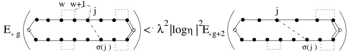
Figure 11: Case 1. Removal of a gate lumped to an adjacent core index
