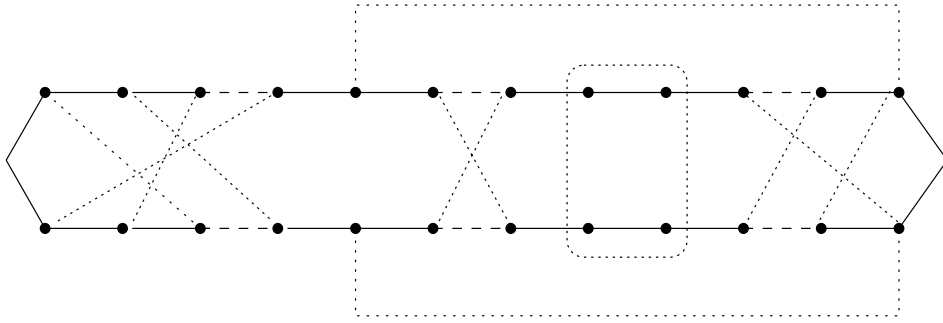
Figure 3: Symmetrized recollision with a gate. \mathbf{D}_0 consists of the paired vertices
