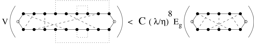
Figure 5: Estimate after removing all non-core indices
