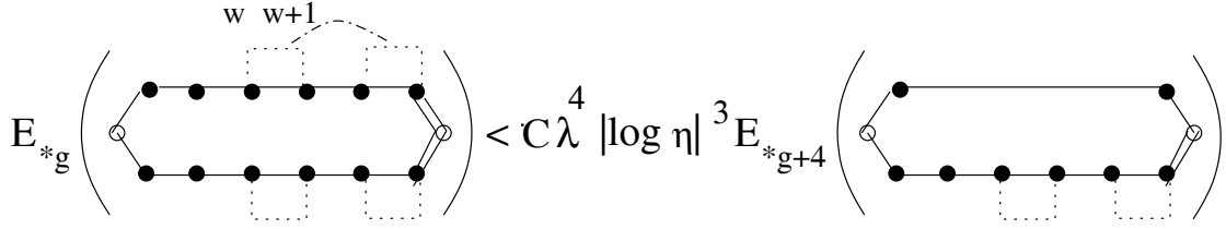
Figure 13: Case 2. Removal of two adjacent lumped gates
