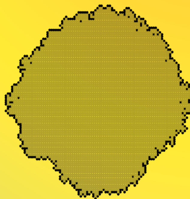
Picture: Lattice Eden growth on \mathbb{Z}^2
