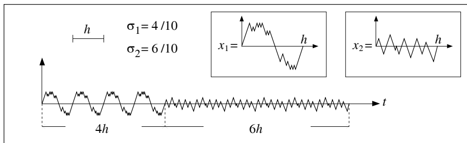
Fig.6. Construction of x for N = 2 , q = 10 , p_1 = 4 , p_2 = 6
