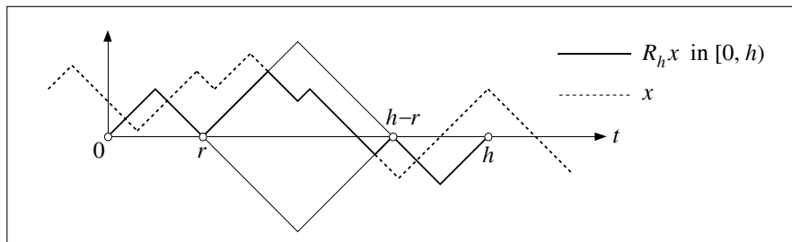
Fig.5. The function R_h x
