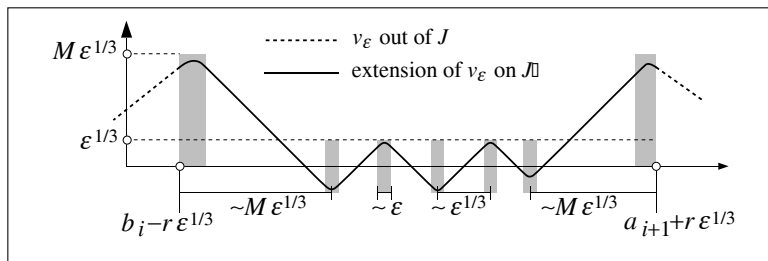
Fig.3. Construction of v^\varepsilon in J := [b_i - r\varepsilon^{1/3}, a_{i+1} + r\varepsilon^{1/3}]
