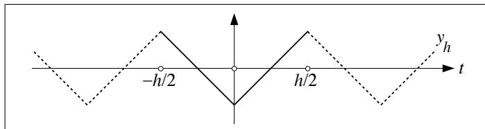
Fig.2. The sawtooth function y_h
