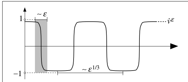
Fig.1. Two scale structure of minimizers
