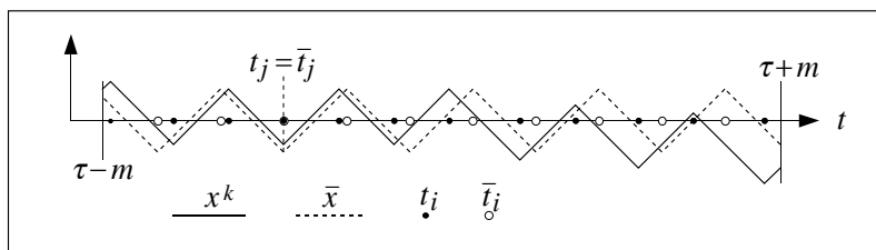
Fig.4. The functions x^k and \bar{x} := T_{t_j} \tilde{x} in (\tau - m, \tau + m)
