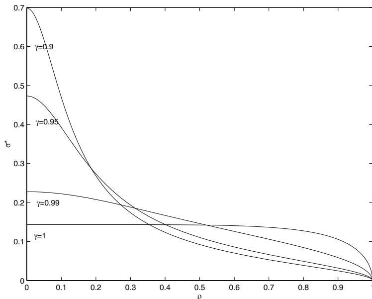
Figure 14: Energy density \sigma^* for \epsilon = 0.8 and several values of \gamma .
