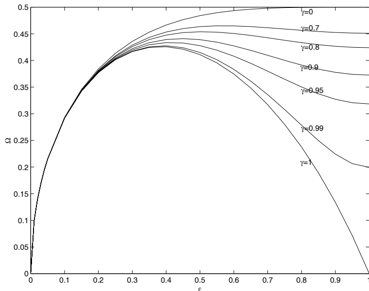
Figure 8: Angular velocity \Omega in dependence of \epsilon for several values of \gamma .
