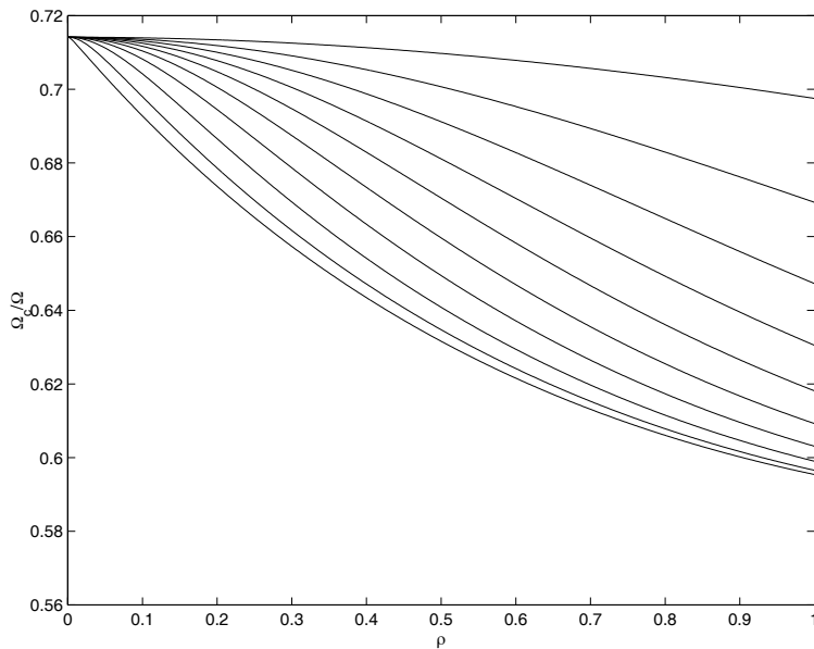
Figure 12: Angular velocity \Omega_c for \gamma = 0.7 and from top to bottom \epsilon = 0.05, 0.15, \dots, 0.95 .
