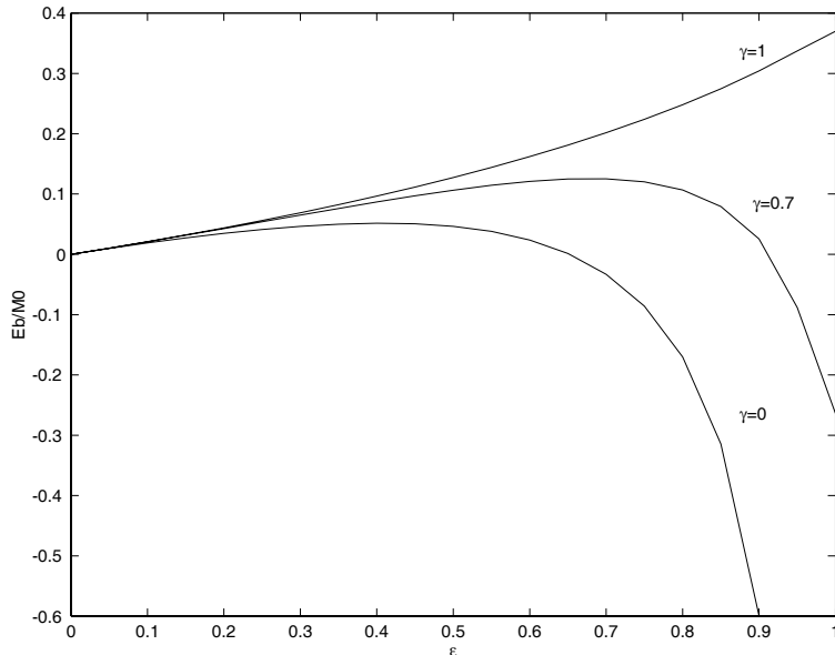
Figure 15: Binding energy of the disks in dependence of \epsilon for several values of \gamma .
