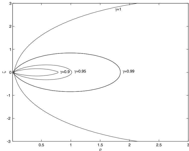
Figure 17: Ergospheres for \epsilon = 0.95 and several values of \gamma .
