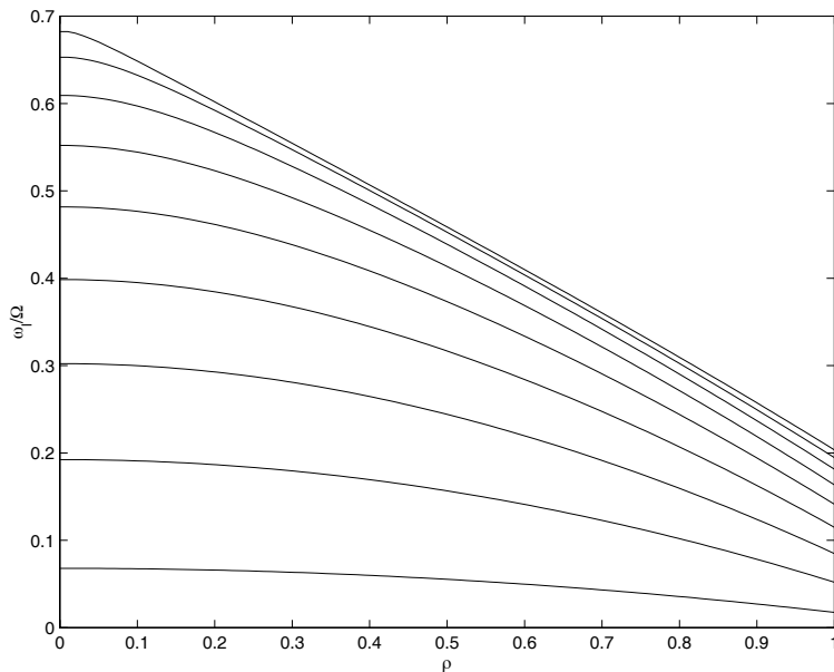
Figure 9: Angular velocity \omega_l for \gamma = 0.7 and \epsilon = 0.05, 0.15, \dots, 0.85 .
