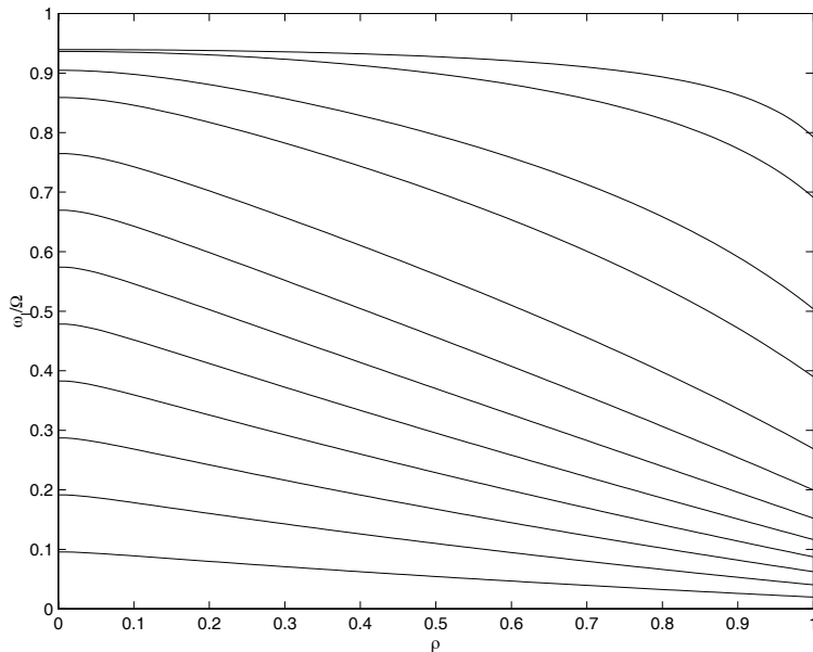
Figure 10: Angular velocity \omega_l for \epsilon = 0.8 and \gamma = 0.1, 0.2, \dots, 0.90.95, 0.99, 1 .
