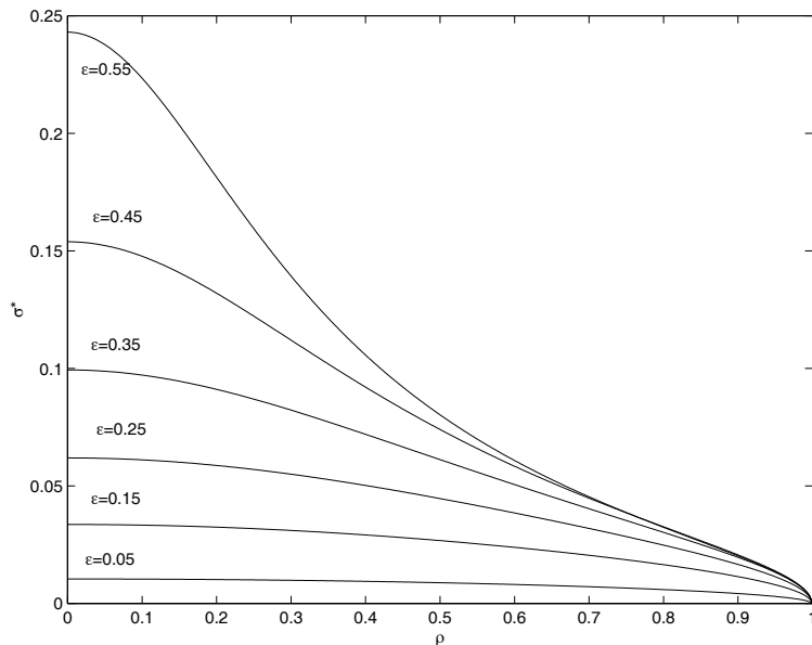
Figure 13: Energy density \sigma^* for \gamma = 0.7 and several values of \epsilon .
