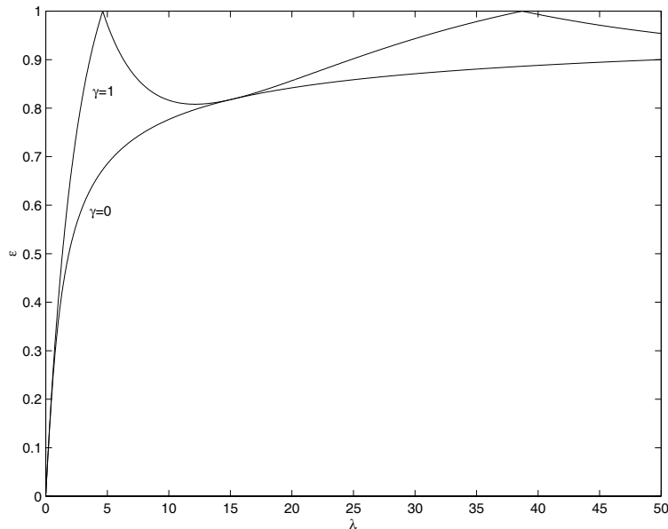
Figure 6: The function \epsilon in dependence of \lambda for \gamma = 1 and \gamma = 0 .
