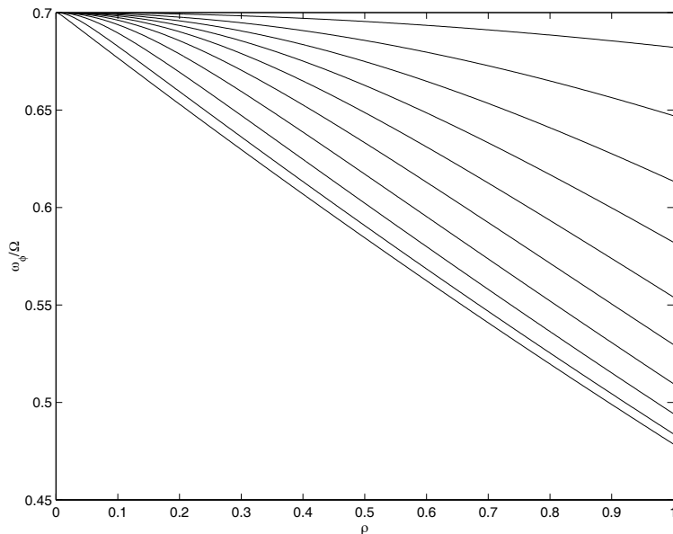
Figure 11: Angular velocity \omega_\phi for \gamma = 0.7 and from top to bottom \epsilon = 0.05, 0.15, \dots, 0.95 .
