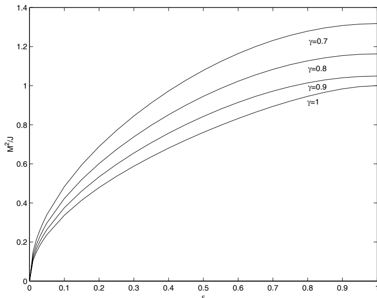
Figure 7: The dimensionless quantity M^2/J in dependence of \epsilon for several values of \gamma .
