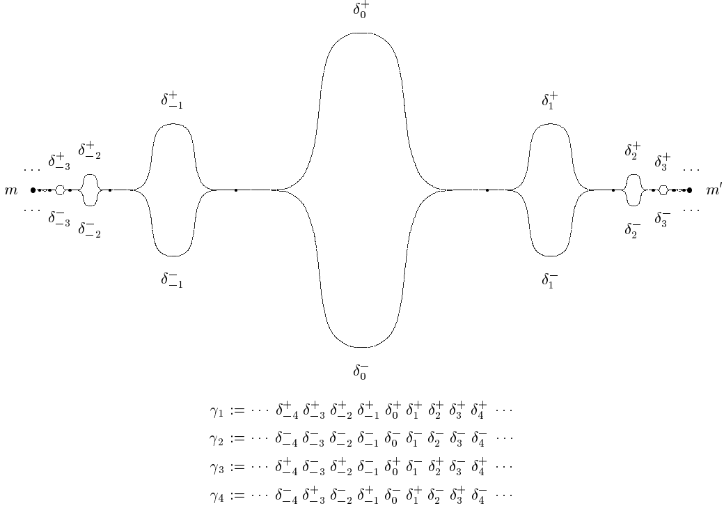
Figure 1: Paths used in the Proof of Lemma 4.7
