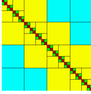
Figure 3.3: \mathcal{H} -matrix structure of the singular-vector Kronecker factors.
