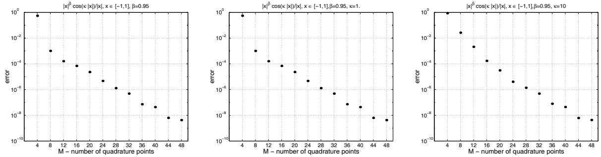
Figure 3.1: Error for the Sinc approximation to F_0 with \kappa = 0.01, 1.0, 10 , respectively, from left to right.
