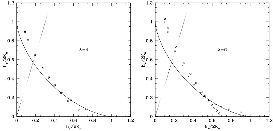
FIGURE 4. Critical fields for cubes with \lambda = 4 (left panel) and \lambda = 6 (right panel), compared with the SW model (full curve). The easy axis is vertical. Circles correspond to points computed in a plane parallel to two faces, crosses to points computed in a plane parallel to two face diagonals (see Figure 3 for the geometry). The other quadrants are symmetric. The dotted lines indicate the direction selected for the plot in Figure 5.
