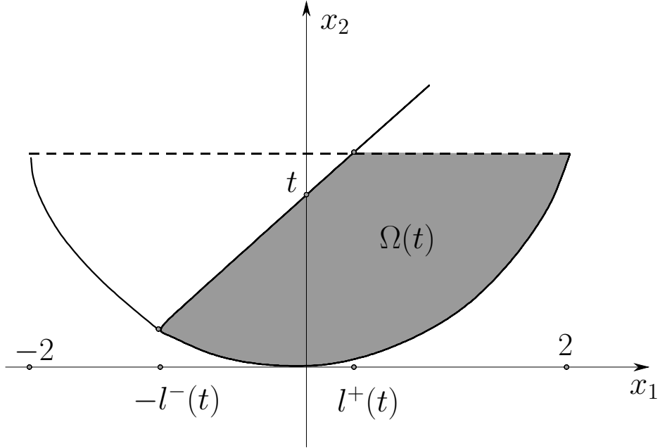
Figure 1: The parabolic domain \Omega and the domains \Omega(t) generated by line segments through the points (0, t)
