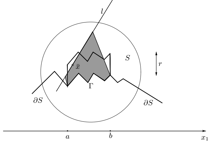
Figure 3: Approximation near the boundary. The Poincaré inequality is applied in the shaded region
