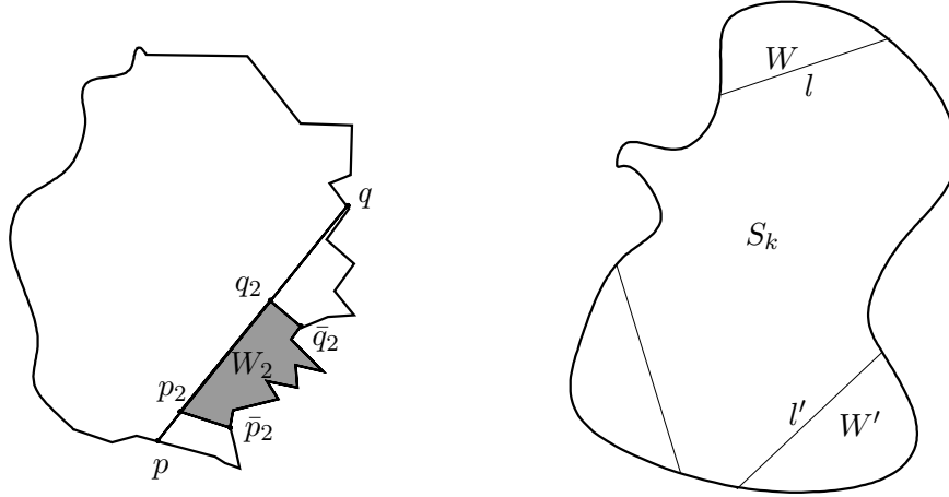
Figure 2: a) Construction of the set W for a long line segment l b) Sets W and W' for different boundary segments l and l' .
