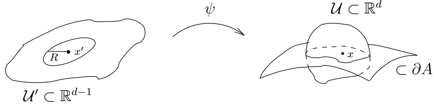
Figure 2: Parameterization of \partial A \cap \mathcal{U} in the proof of Proposition 5.
