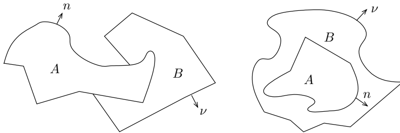
Figure 1: Sketches of possible configurations.
