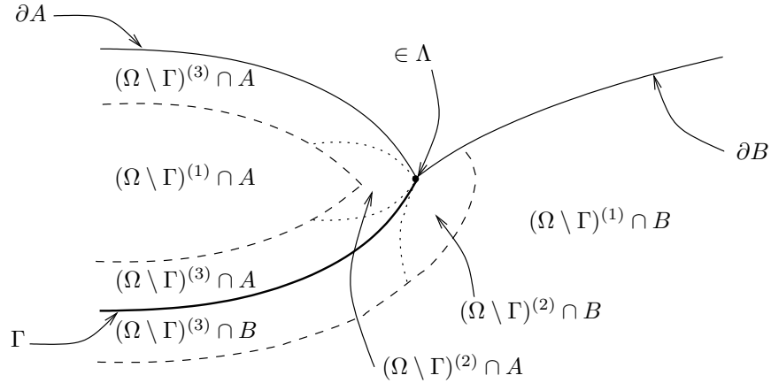
Figure 3: Sketch of the sets (\Omega \setminus \Gamma)^{(1)} , (\Omega \setminus \Gamma)^{(2)} and (\Omega \setminus \Gamma)^{(3)} as defined in the proof of Theorem 15. In this sketch we consider a geometric setting where (a portion of) \Lambda happens to be in the relative boundary of \Gamma .
