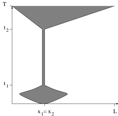
FIGURE 3. Phases \{u_k = 1\}
