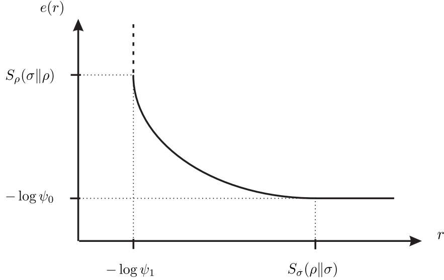
Figure 2: Example plot of the quantum error-exponent function e_Q(r) in the general case.
