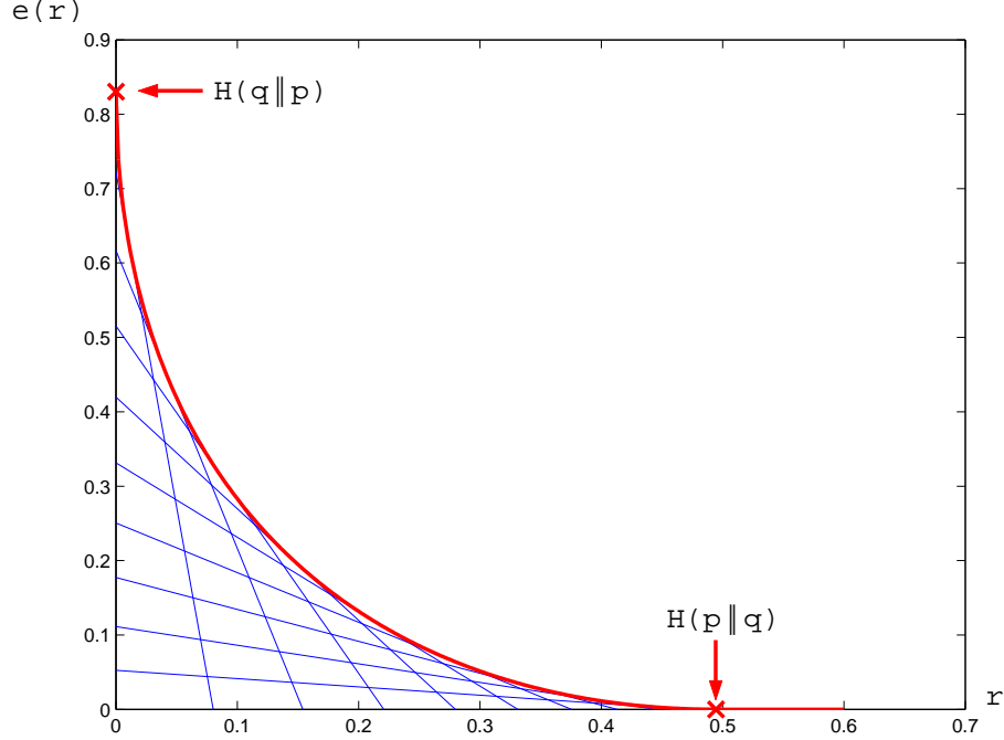
Figure 1: (Color online) Example plot of the error-exponent function e(r) , eq. (42), for the distributions p = (0.95, 0.05) and q = (0.5, 0.5) . The thick (red) line is the graph of e(r) , while the thin (blue) lines are instances of the linear function (-rs - \log \sum_k q_k^s p_k^{1-s}) / (1-s) for various values of s , of which e(r) is the point-wise maximum. For the chosen p and q , the value of H(p||q) = 0.49463 and the value of H(q||p) = 0.83037 .
