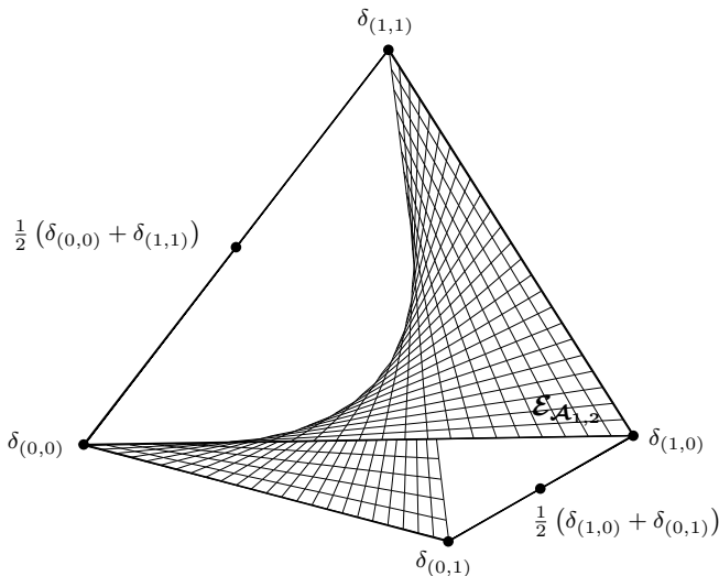
FIGURE 1. The exponential family \mathcal{E}_{\mathcal{A}_{1,2}} in the simplex of probability distributions.
