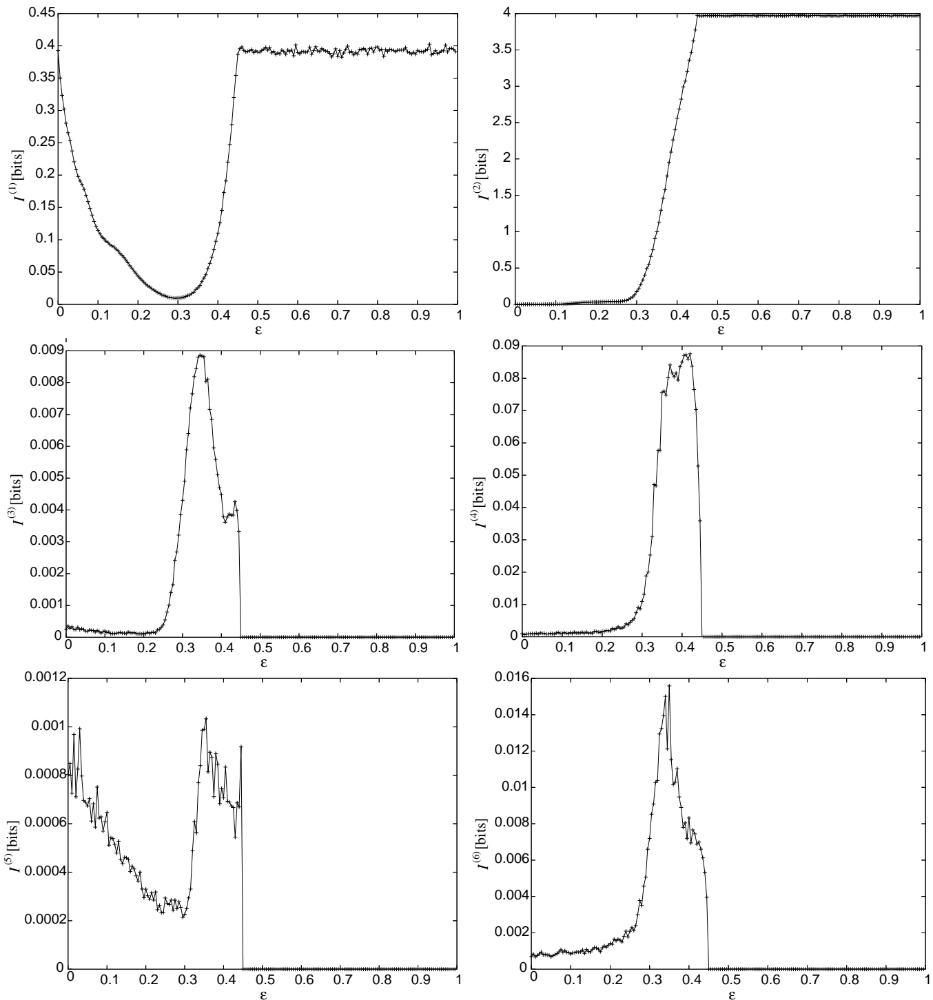
FIG. 5: The Values of I^{(k)} for the fully connected graph. For \epsilon > 0.45 , the network is in the state of synchronized chaos. This is fully captured by pair interactions, therefore I^{(2)} is maximal, while the I^{(k)} for k > 2 vanish. On the edge to synchronized chaos high correlations on different scales are detected.
