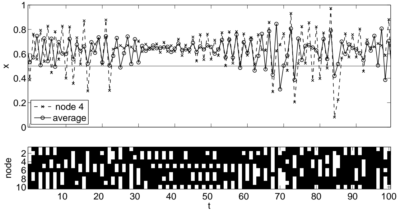
FIG. 3: A snapshot of the complex dynamic of the circle graph at \epsilon = 0.482 . In the top the activity of node 4 is plotted together with the average activity over all nodes. One can observe that for short periods of time synchronization effects occur, for instance between t = 30 and t = 40 node 4 is almost constant while the average also fluctuates less. Below the symbolic dynamics, with black as one, white as zero, of all 10 nodes is shown. The synchronization is visible here too as the pattern after t = 35 is very regular.
