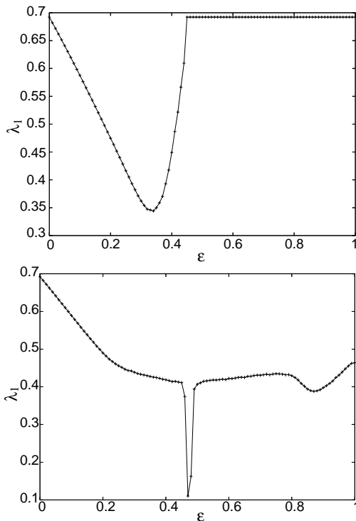
FIG. 4: Behavior of the largest Lyapunov exponent \lambda_1 for the fully connected graph(top), and the circle graph(bottom). Note that the minima are attained in exactly the same parameter region, in which the I^{(k)} have maxima.
