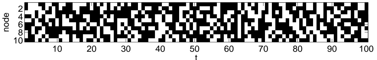
FIG. 2: A snapshot of the weakly coupled chaotic dynamic of the circle graph at \epsilon = 0.04 . Each row shows one node over time. White spots indicate the value zero, black squares one.
