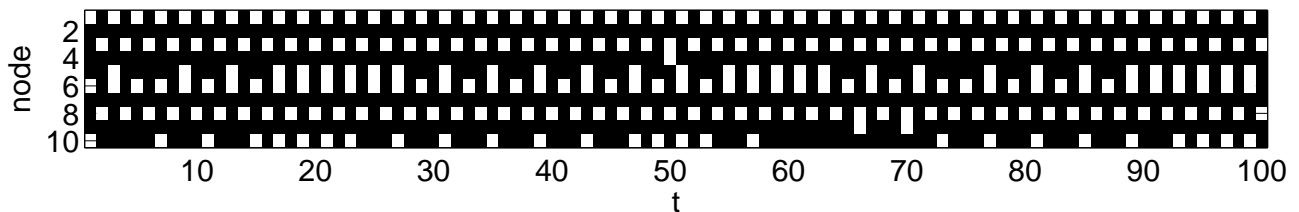
FIG. 1: A snapshot of the highly regular binary symbolic dynamics of the circle graph at \epsilon = 0.476 . Each row shows one node over time. White spots indicate the value zero, black squares one.
