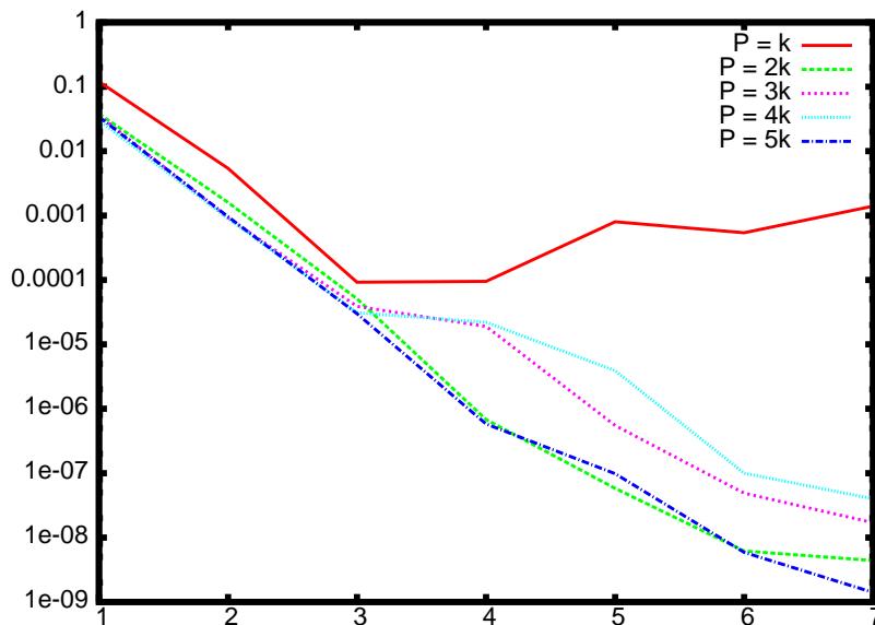
Figure 3: Approximation error (in log-scale) for different numbers of pivot indices P = c_P k in dimension d = 4 .
