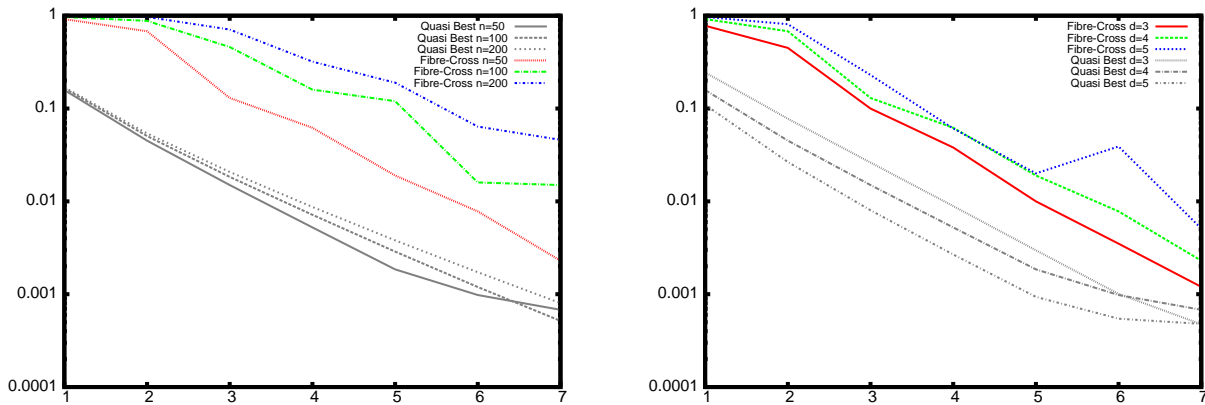
Figure 5: The decay of the relative error for a rank k = 1, \dots, 7 approximation for varying meshwidth (left) and varying dimension (right).
