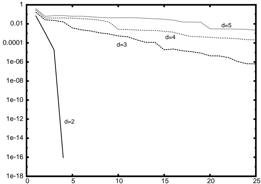
Figure 2: The relative error \epsilon = \|A - X\|/\|A\| in log-scale of a pure cross approximation with k = 1, \dots, 25 terms in d = 2, \dots, 5 .
