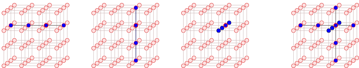
Figure 1: The index sets J^{p,1}, J^{p,2}, J^{p,3} for the pivot index I^p := (3, 3, 3) , and the whole fibre-cross (in d = 3 ).
