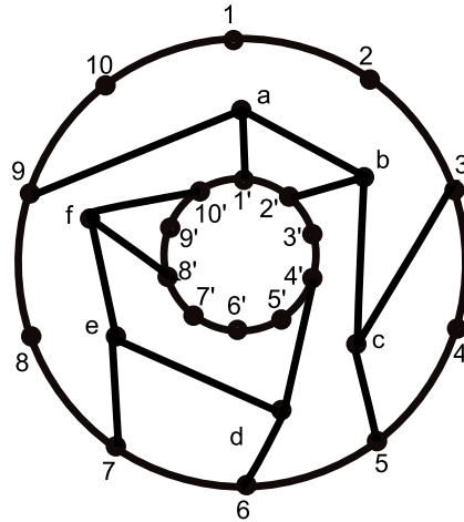
Figure 4: (4,8,8) in \mathbb{R}P^2
