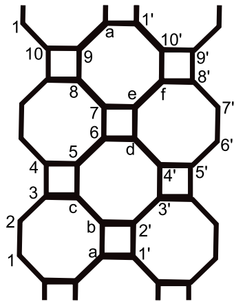
Figure 3: (4,8,8)
