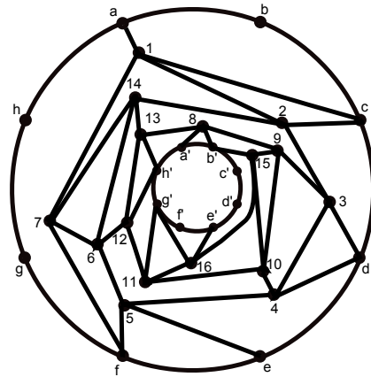
Figure 6: (3,4,6,4) in \mathbb{R}P^2
