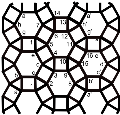
Figure 5: (3,4,6,4)
