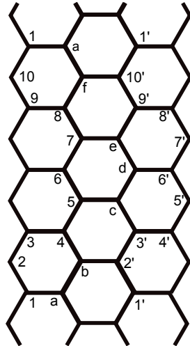
Figure 1: (6,6,6)
