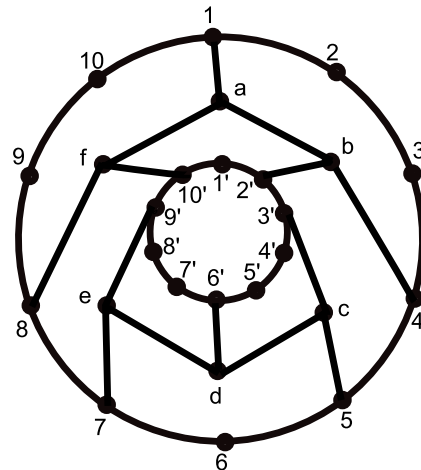
Figure 2: (6,6,6) in \mathbb{R}P^2
