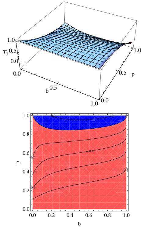
FIG. 1. (Color online) Here we select A_i = U_2\sigma_iU_2^\dagger , B_i = V_2\sigma_iV_2^\dagger , C_i = \sigma_i , with U_2 = |0\rangle\langle 1| - |1\rangle\langle 0| , V_2 = \frac{1}{\sqrt{2}}(|0\rangle\langle 0| + |0\rangle\langle 1| - |1\rangle\langle 0| + |1\rangle\langle 1|) , i = 1, 2, 3 . The first plot describes expectation value \langle T_1 \rangle_{\rho_3} with respect to p and b . The second plot is the contour plot of the first.
