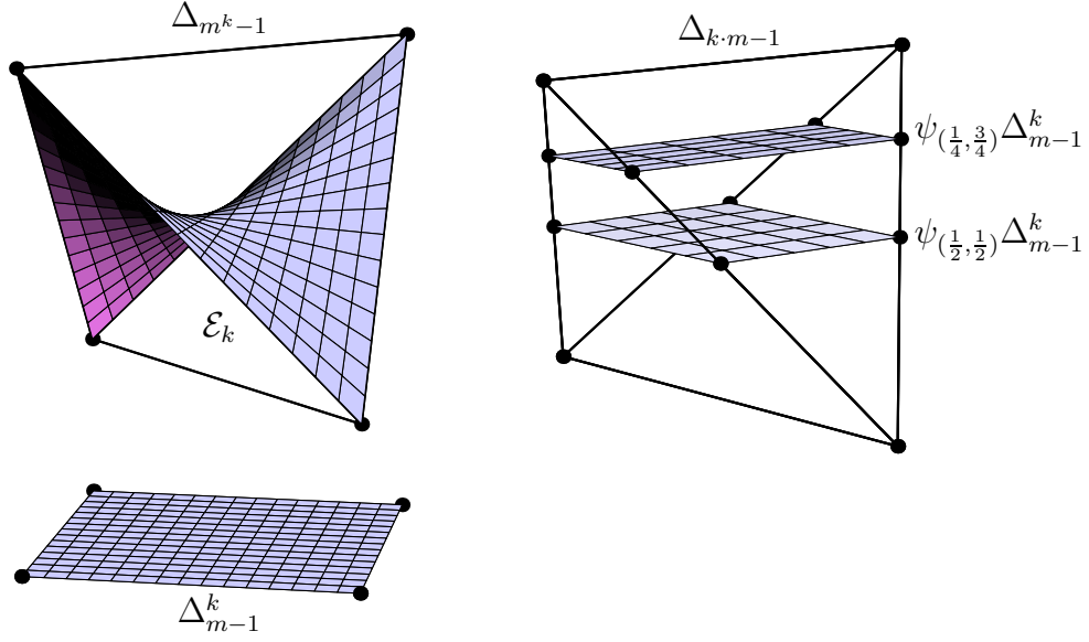
Figure 2: An illustration of different embeddings of the conditional polytope \Delta_{m-1}^k in a probability simplex. The left panel shows an embedding in \Delta_{m^{k-1}} by the inverse of the moment map \mu of the independence model. The right panel shows an affine embedding in \Delta_{k,m-1} as a set of joint probability distributions for two different specifications of marginals.
