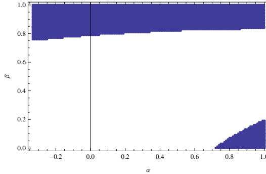
Figure 3: (Color on line) Quantum states \rho parameterized by (\alpha, \beta) that admit no LHV model (blue regions).
