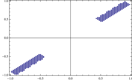
Figure 2: The same cross-sectional view of Fig. 1 for all p_1 = 0.9 , p_2 = 0.9 and p_3 = 0.9 .
