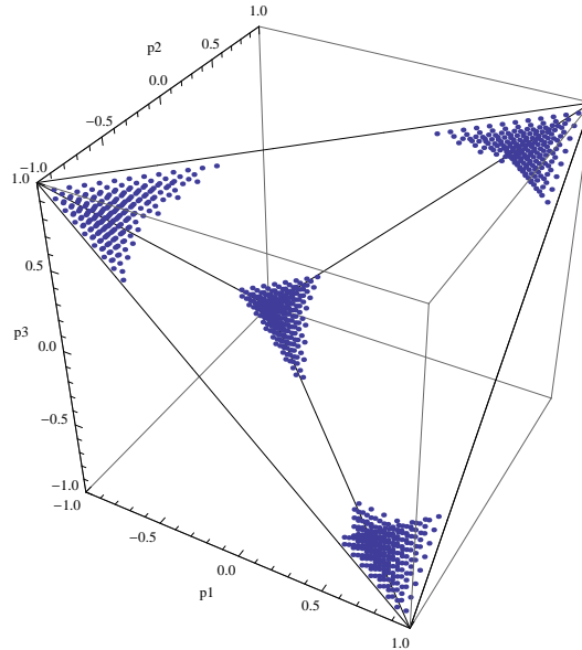
Figure 1: The quantum states \rho_w that admits no LHV models are listed by the points parameterized by (p_1, p_2, p_3) .
