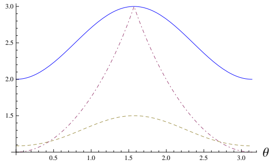
Figure 2: The blue solid line is the sum of the variances (\Delta\sigma_1)^2 + (\Delta\sigma_2)^2 + (\Delta\sigma_3)^2 . The dot-dashed line is the bound (3). The dashed line is the bound (6).
