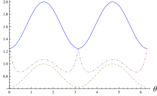
Figure 1: The blue solid line is the sum of the variances (\Delta\sigma_1)^2 + (\Delta\sigma_3)^2 . The dot-dashed line is the bound (3). The dashed line is the bound (4).
