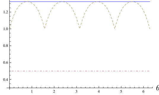
Figure 3: The blue solid line is the uncertainties \Delta\sigma_3\sqrt{(\Delta\sigma_2)^2 + (\Delta\sigma_1)^2} . The dot-dashed line is the bound (9). The dashed line is the bound (8).
