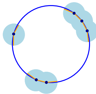
FIGURE 2. Six points whose t -neighborhood has no cycle.
